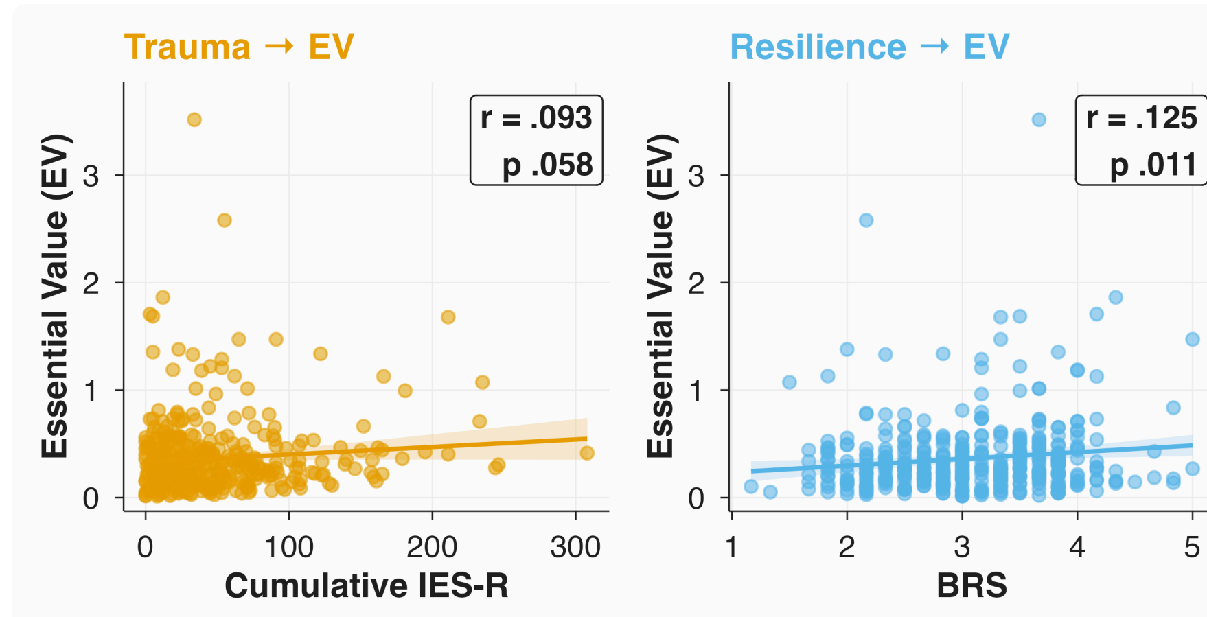
Figure 3 · Essential Value plotted against cumulative trauma (left) and resilience (right). Points represent participants; the line is a linear fit with 95% CI; Pearson r is shown in each panel. (N = 415).
